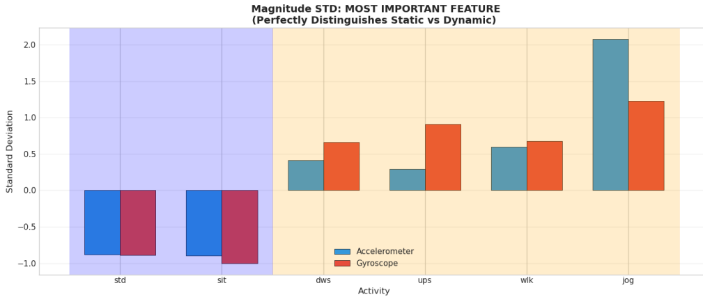
Figure 6: Comparison of Standard Deviation between Accelerometer and Gyroscope magnitudes. Gyroscope signals provide a more distinct separation for identifying movement intensity due to lower gravitational interference.
